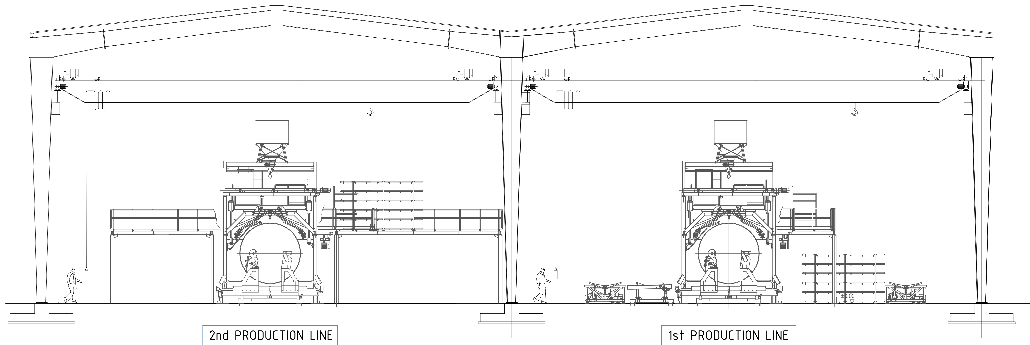
PRODUCTION SHEDS SIDE VIEW
