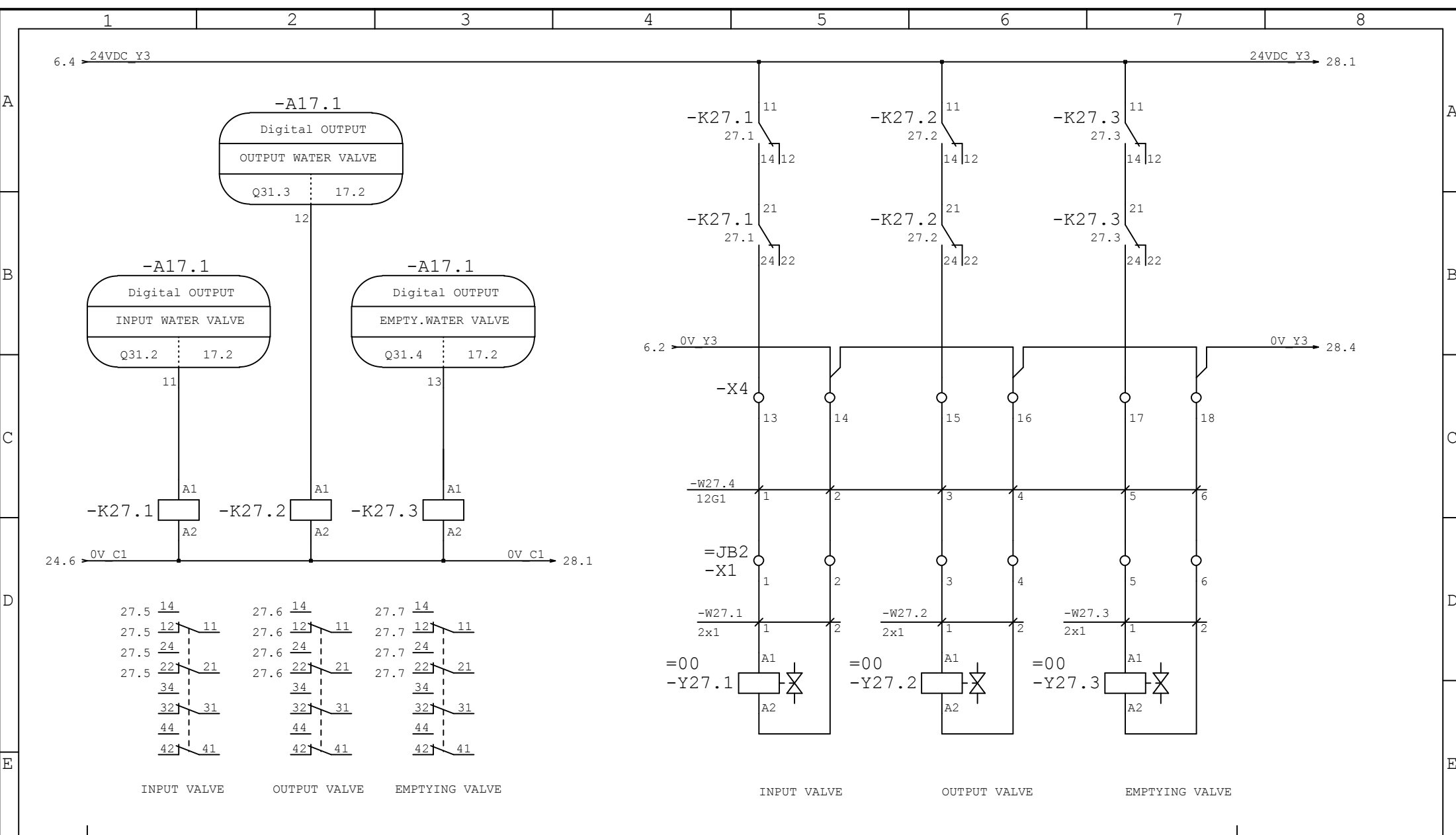
MOULD - HIGH PRESURE WATER VALVES
